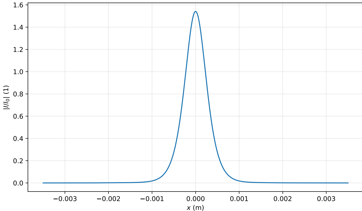
Intensity profile I(x, y = 0, z = 3.184m)/I_0 , P_{in}=0.9P_{cr} , artificial time
